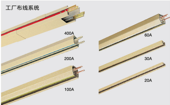
Duct System
